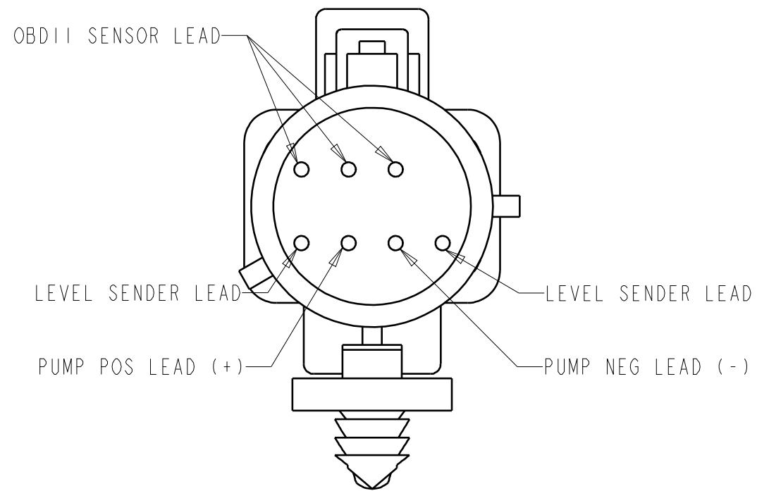
CONNECTOR MODULE MAIN PINOUT DETAIL SCALE 2:1
